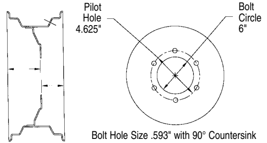
Bolt Hole Size .593" with 90° Countersink
